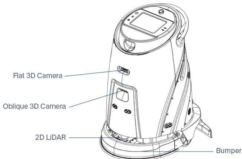
Figure 1: Scrubber 50 Sensors
